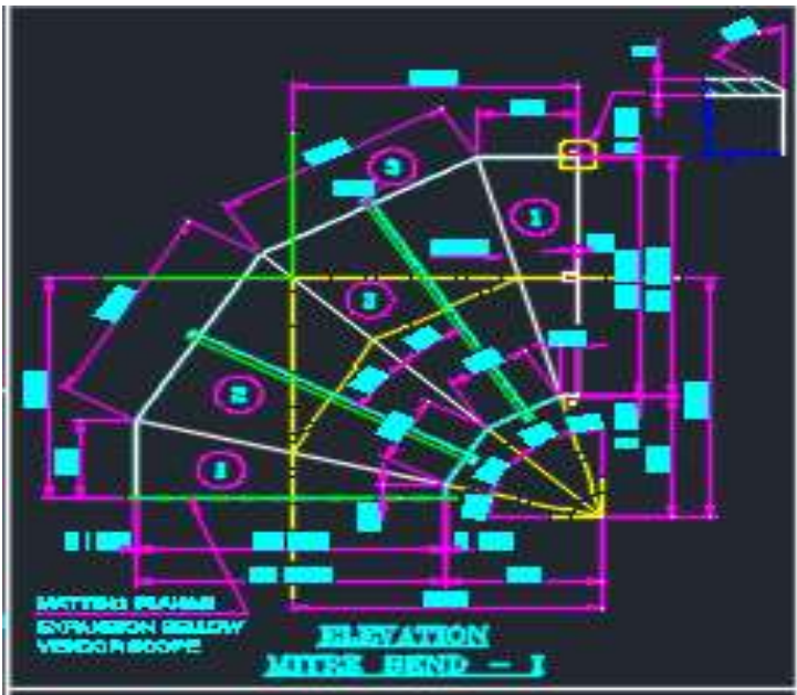
Duct
