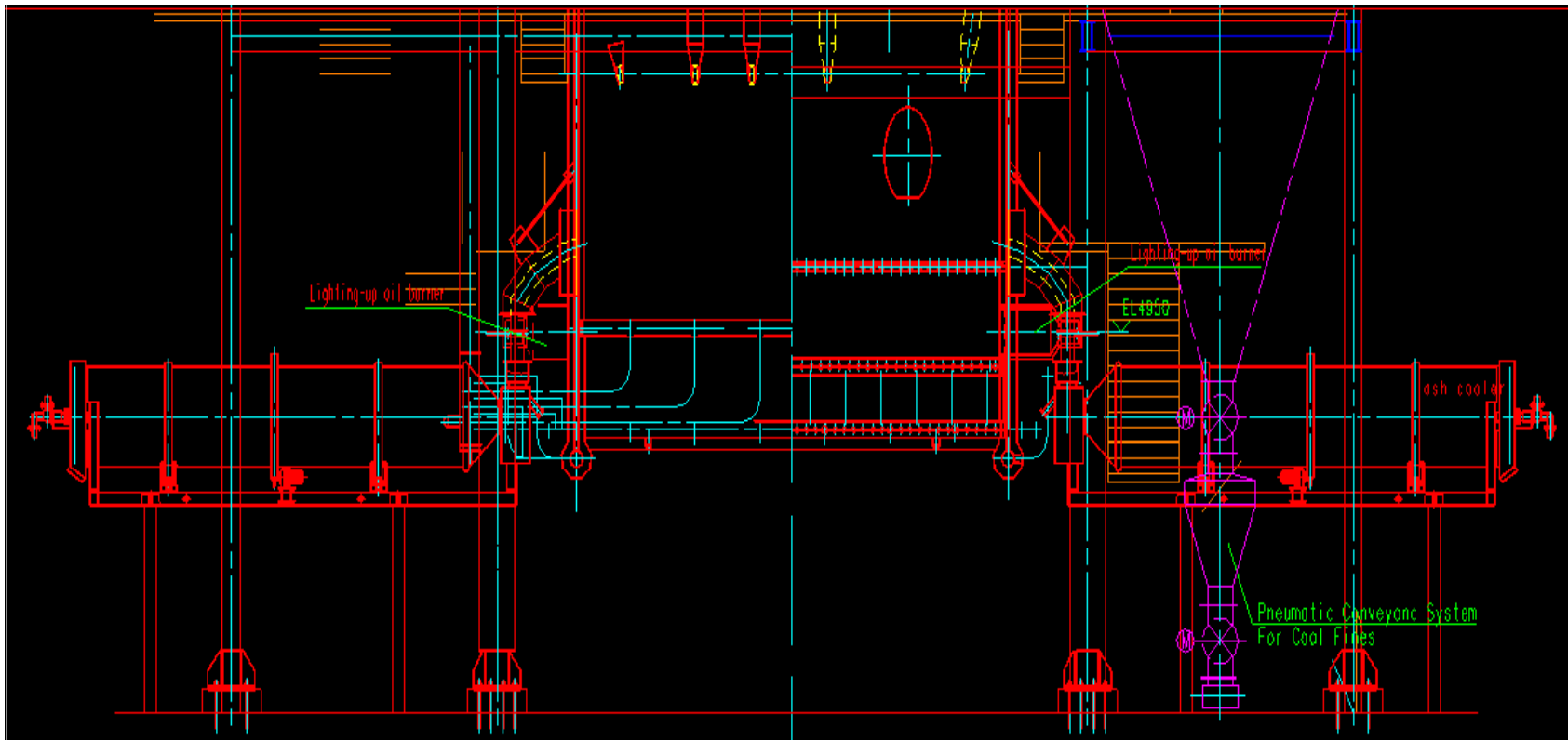
Existing CFB Boiler Rotary Ash cooler System
